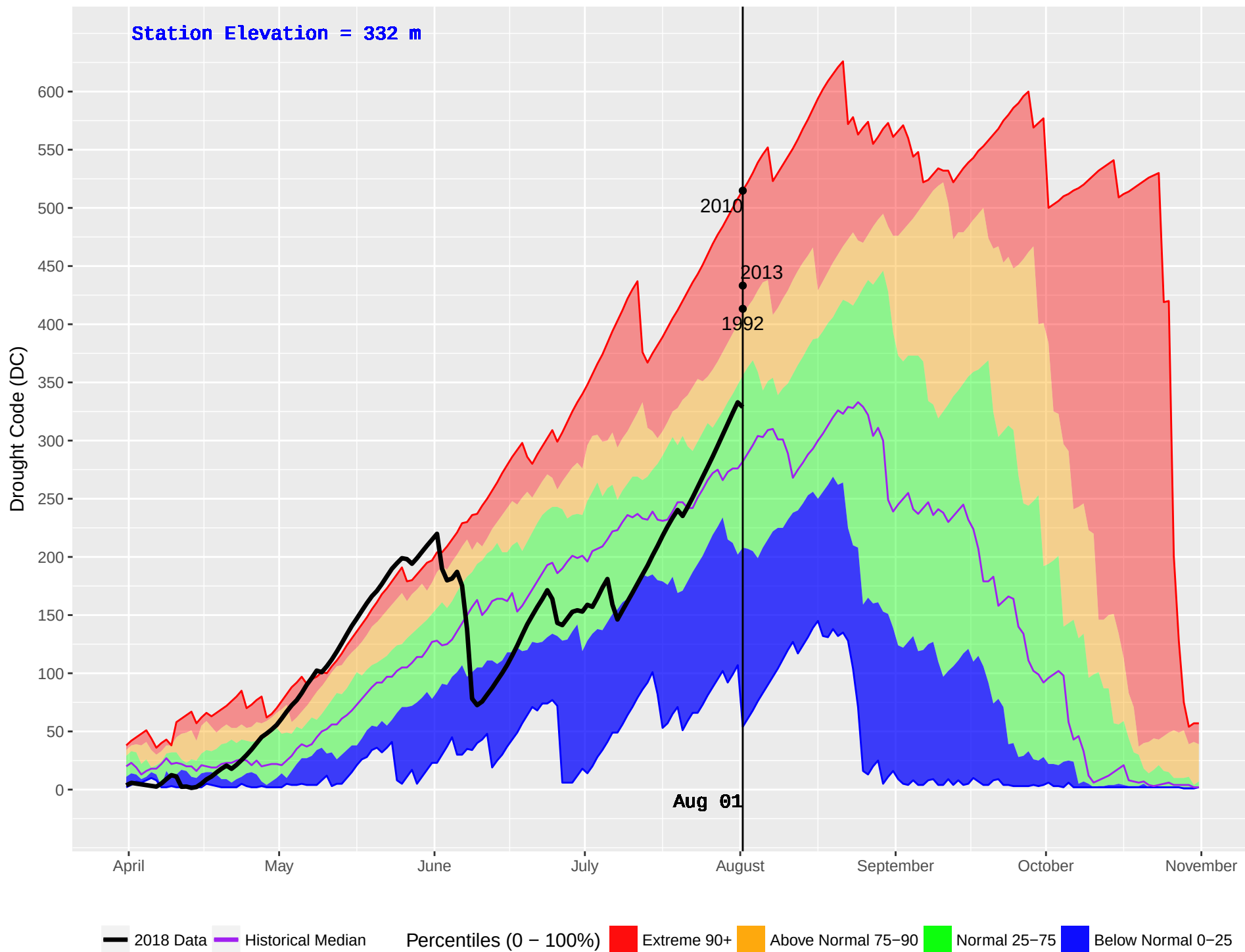
MACHMELL (101) : Historical (1990–2016) and Current (2018) Daily Drought Code (DC)
