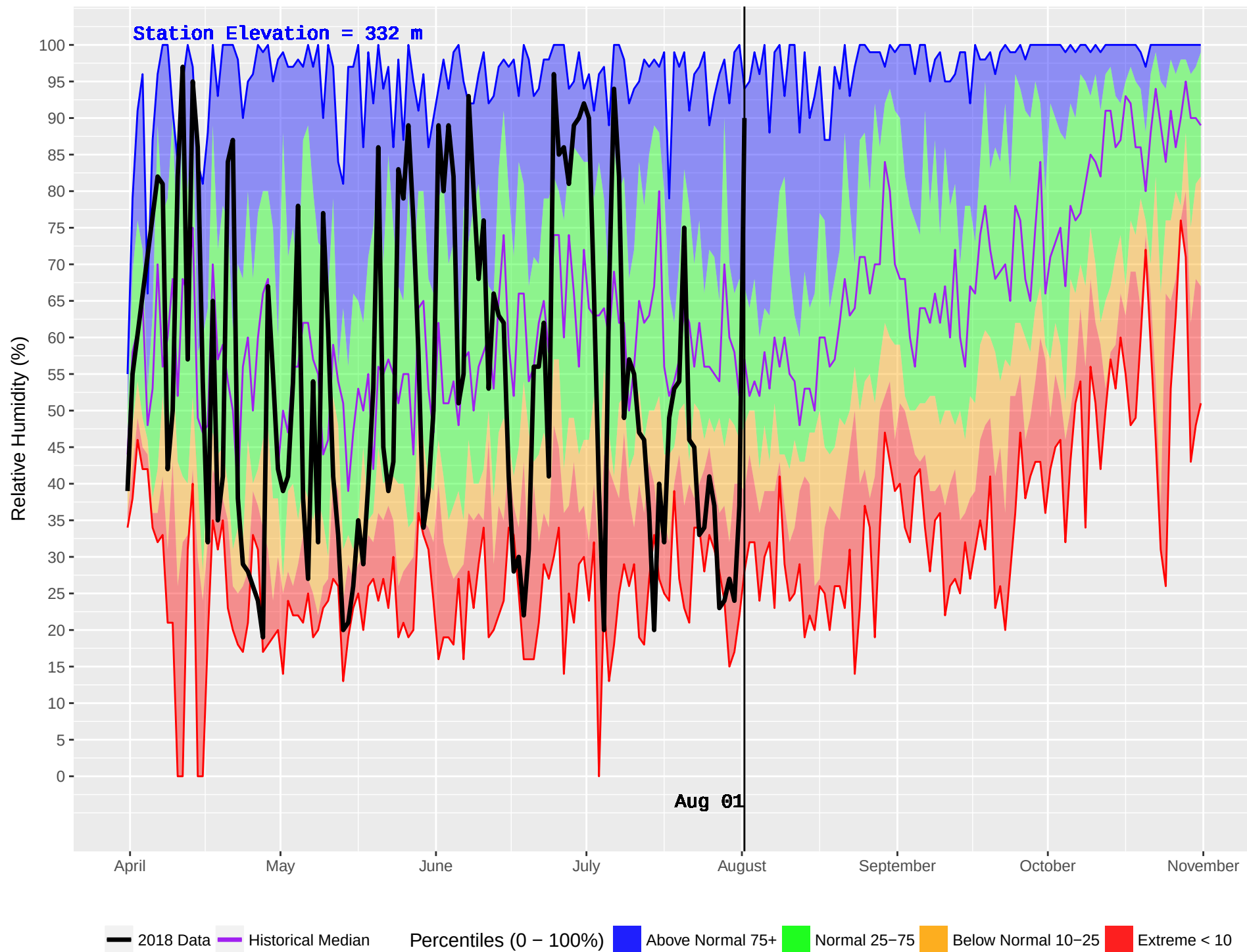
MACHMELL (101) : Historical (1990–2016) and Current (2018) Daily Relative Humidity
